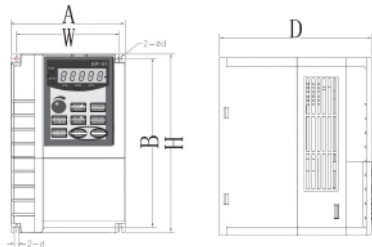
PD ES IP 20 protection level dimensions
