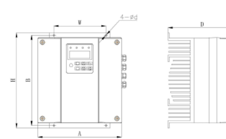
PD ES IP 65 protection level dimensions
